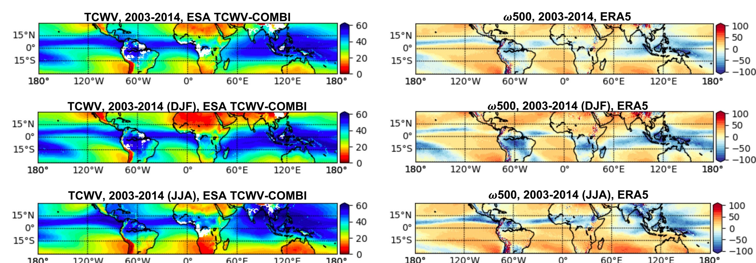
Fig. 1. Maps of the ESA TCWV-COMBI (in kg/m²) during 2003 - 2014 for the tropical region (30°S - 30°N) for the whole period, Winter (December, January and February - DJF), and Summer (June, July, and August - JJA) and the corresponding maps of ERA5 \omega_{500} (in hPa/day).
